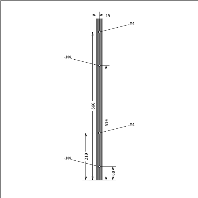
DRAWING 1, Pos 4 SIDE 1, bar length: 720.0 mm
